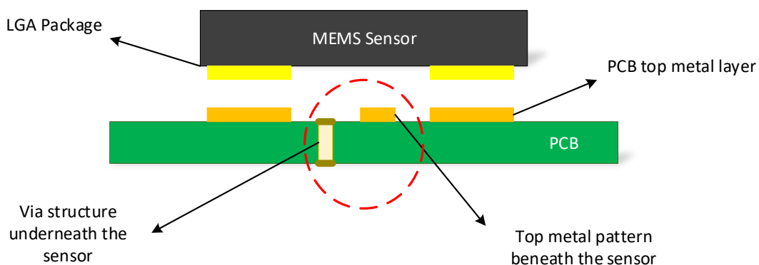
Figure 12: Incorrect PCB design
