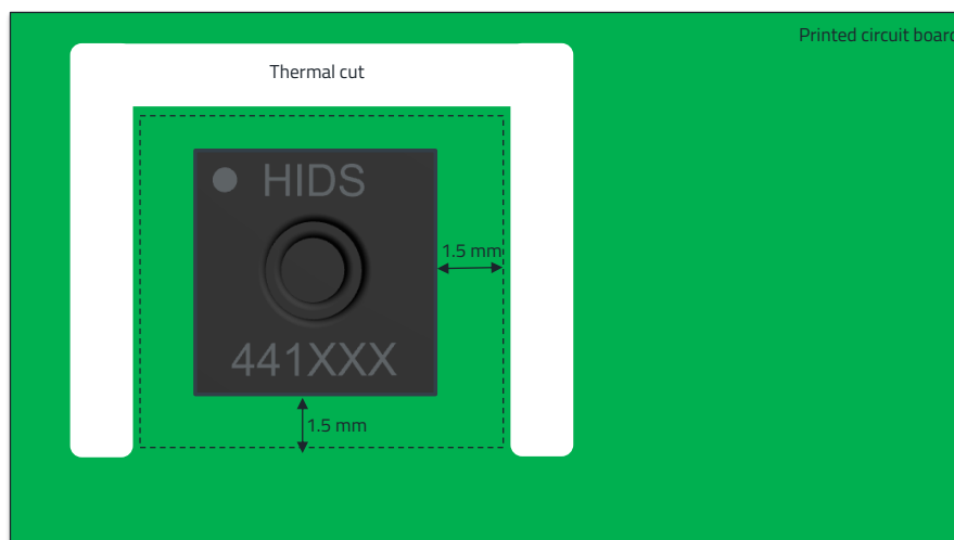
Figure 16: Thermal cut around the sensor
