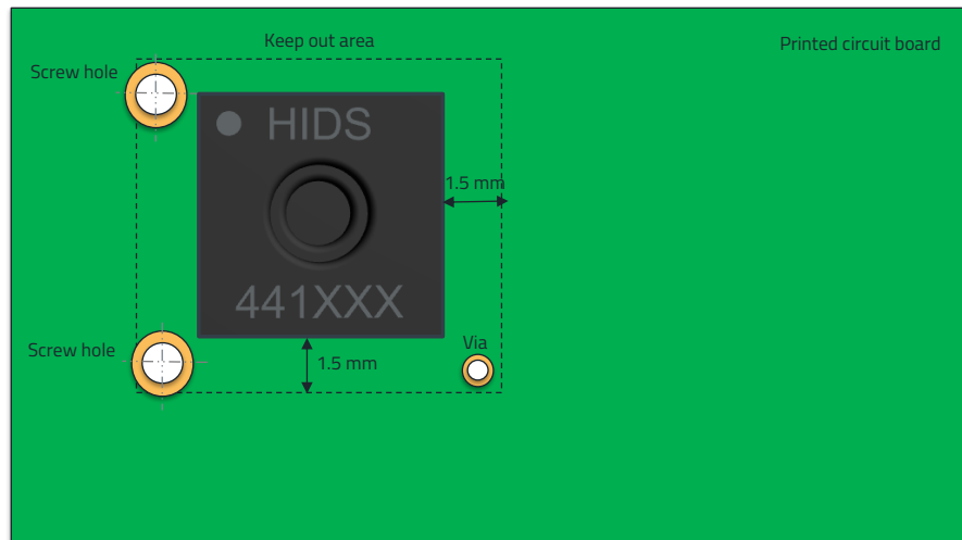
Figure 14: Components inside sensor keep out area
