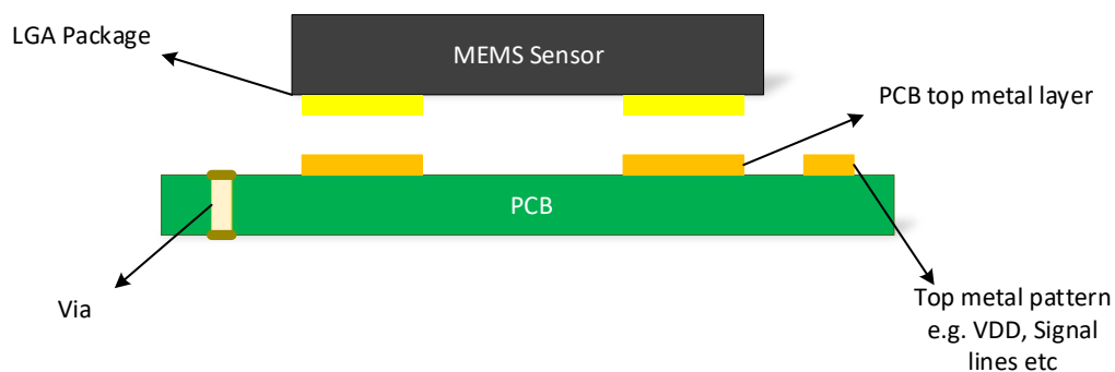
Figure 13: Correct PCB design
