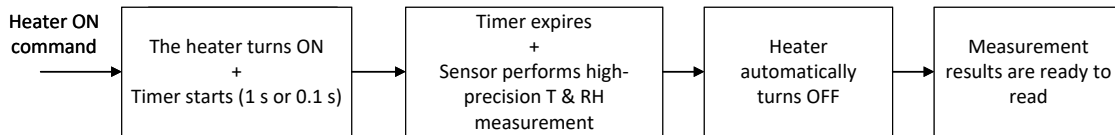
Figure 8: Sensor heater operation
