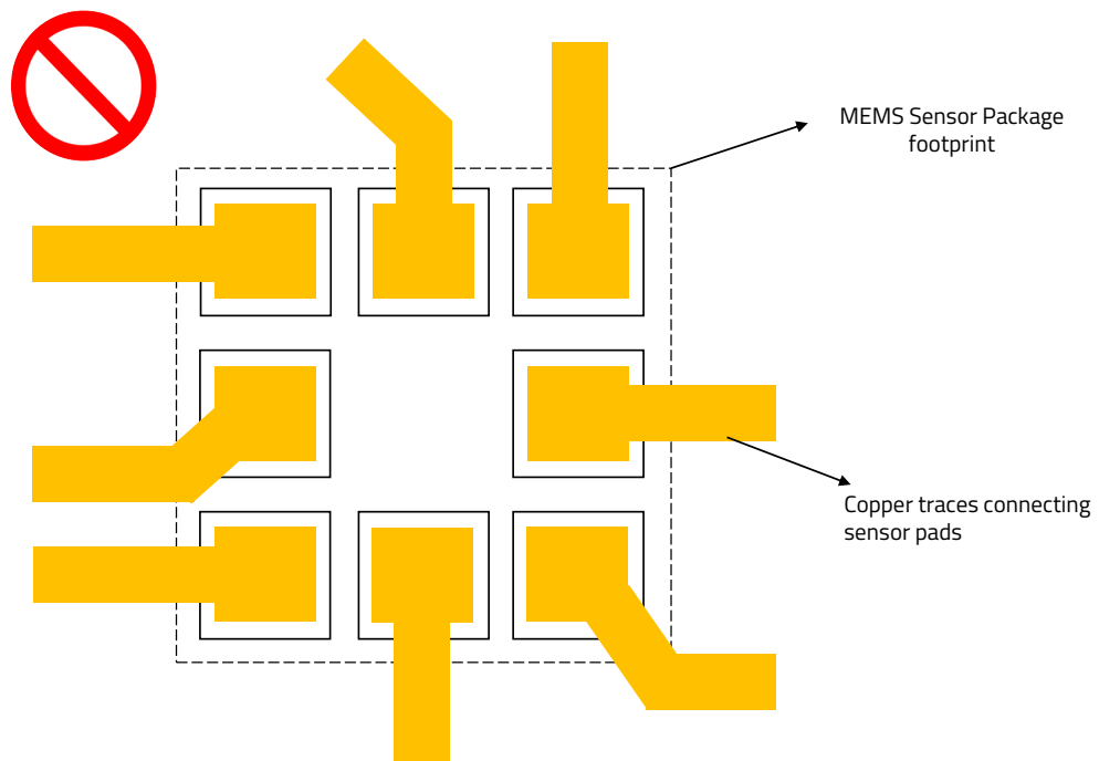
Figure 17: Asymmetrical trace and sensor pad connections
