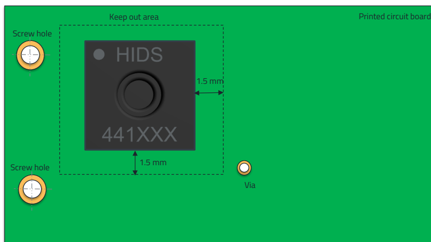
Figure 15: Components outside sensor keep out area
