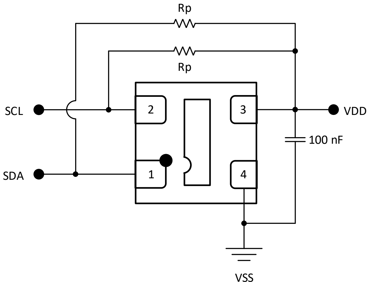
Figure 3: Electrical connection
