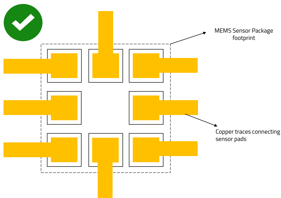
Figure 18: Symmetrical trace and sensor pad connections
